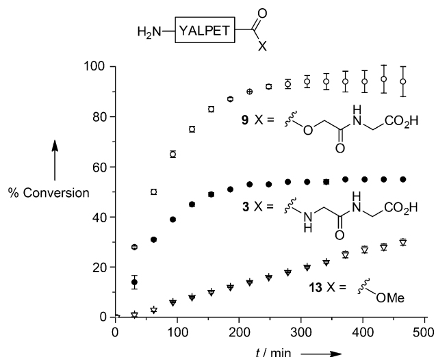
Figure 2. Time-course of SrtA-mediated ligation of 3, 9 and 13 with 4 at a 1:1 ratio at 37°C. 500 \mu M 4 and 500 \mu M 3, 9 or 13 with 11 \mu M SrtA in 50 mM HEPES, 5 mM CaCl 2 150 mM NaCl pH 7.5.
